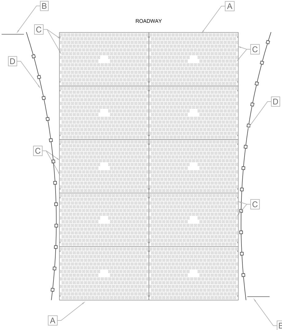
TYPICAL ENTRANCE LAYOUT
