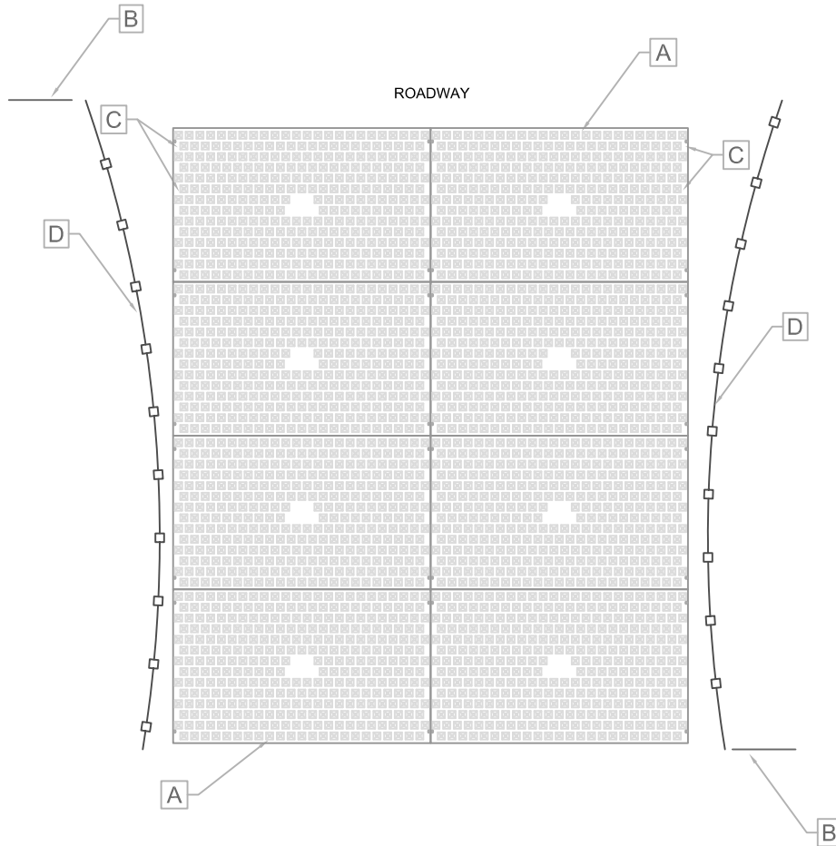
TYPICAL ENTRANCE LAYOUT
