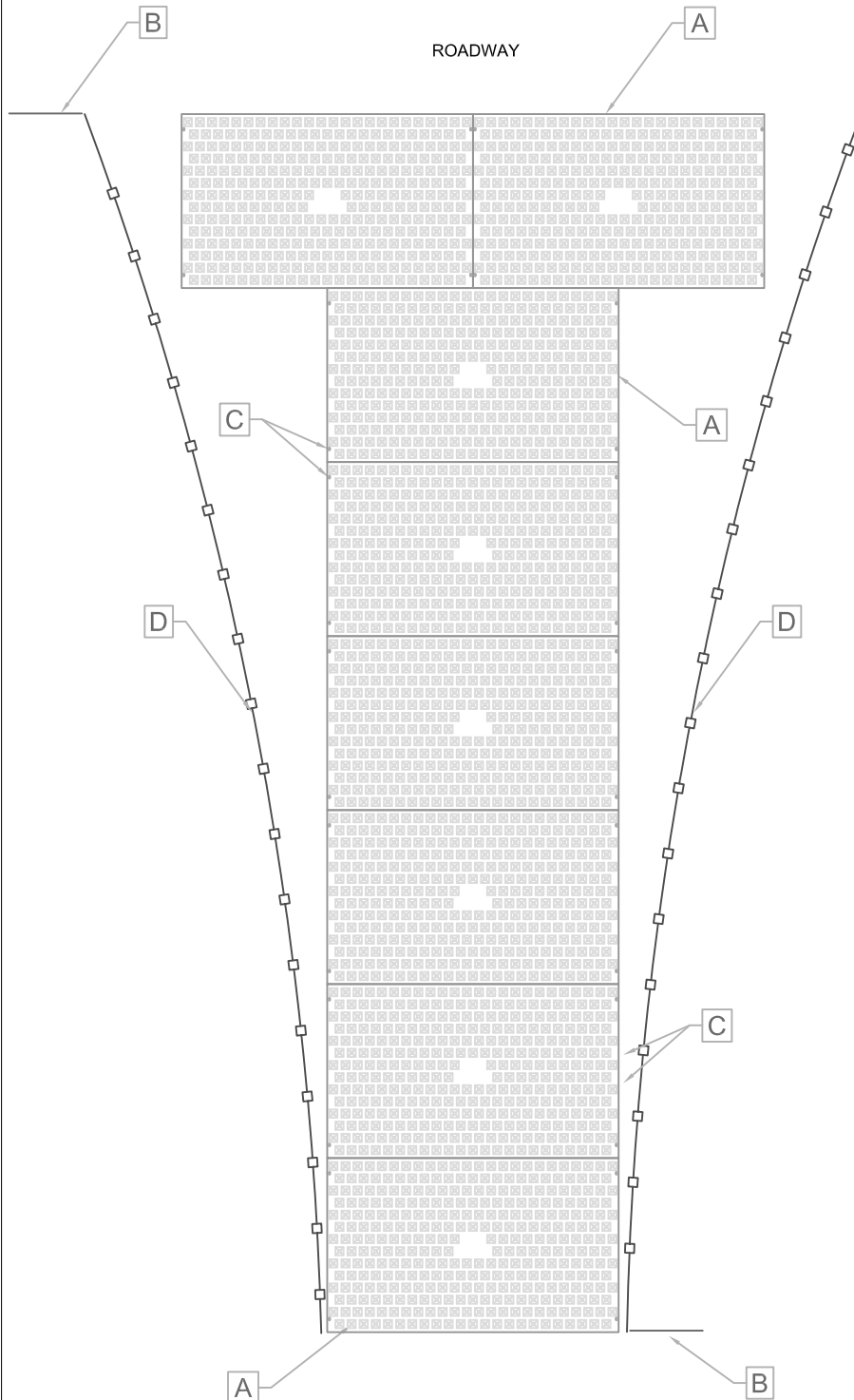
TYPICAL ONE-LANE LAYOUT
