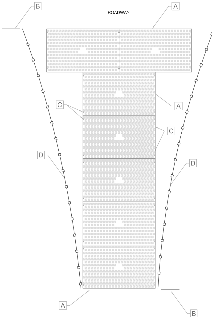
TYPICAL ONE-LANE LAYOUT
