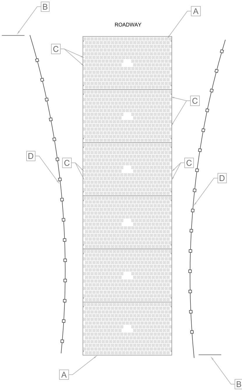
TYPICAL ONE-LANE LAYOUT
