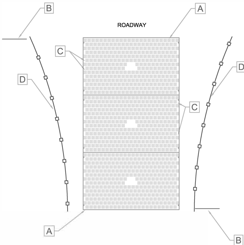
TYPICAL ONE-LANE LAYOUT
